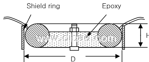
O-core power transformer
